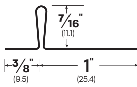
Plain Rib Strip 1-3/8" Base MATERIALS: BR, ZN
