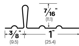
Side Strip 1-3/8" Base MATERIALS: BR
