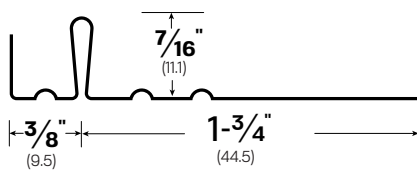
Side Strip 2-1/8" Base MATERIALS: BR, ZN
