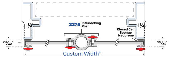
#5129 MOUNTED TO OUTSIDE OF FRAME
