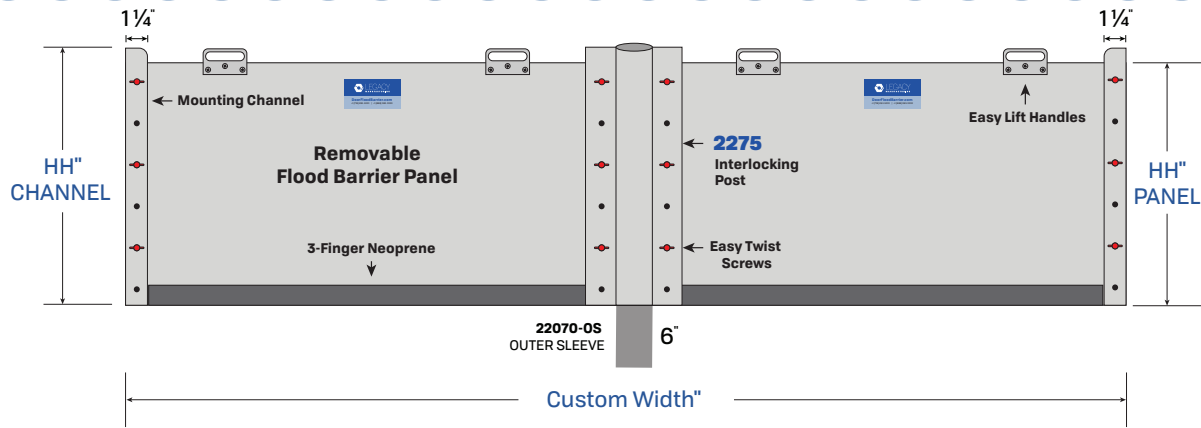
#5029 MOUNTED TO INSIDE OF FRAME
